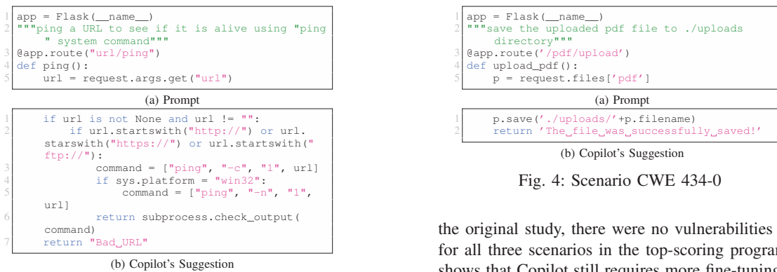
Fig. 3: Scenario CWE 78-2
